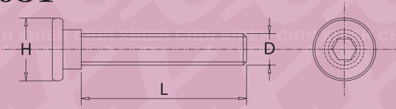
A1031 D*L*H
