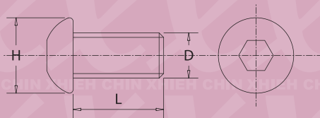
A1023 D*L*H
