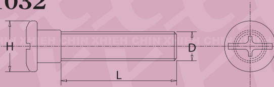
A1032 D*L*H
