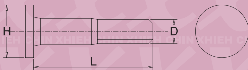
A1046 D*L*H
